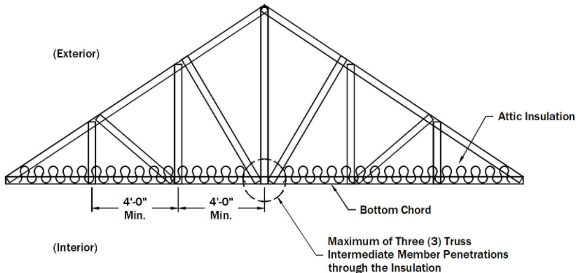
Figure C-B4.1-1 Standard Truss Framing in Roof/Ceiling Assembly
