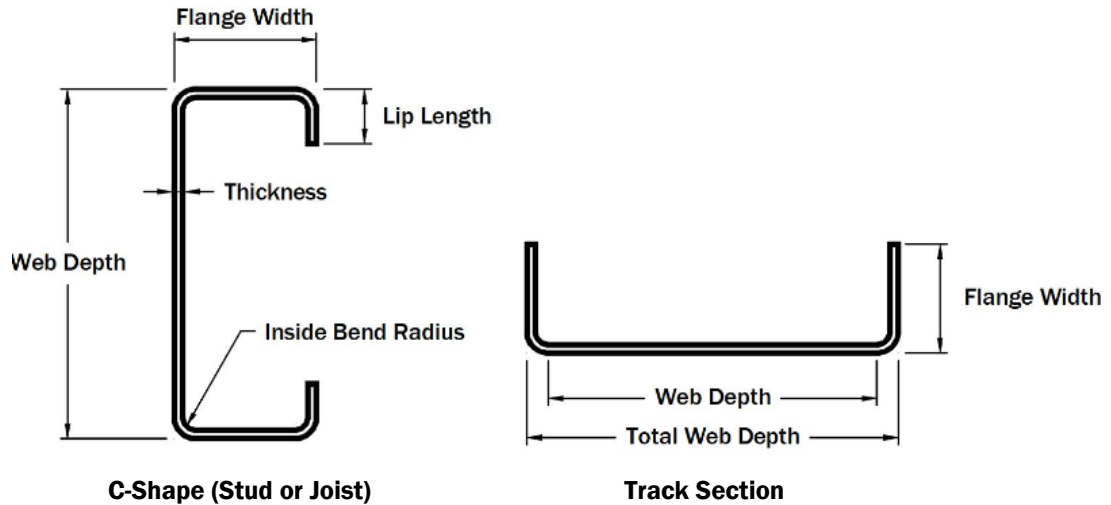
Figure C-A2-1 Standard Cold-Formed Steel Framing Members
