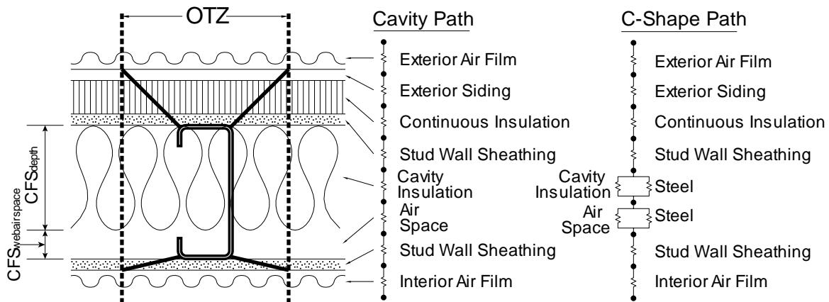
Figure B3.1.3-2 Wall Assembly and Circuit Diagram - With Cavity Air Space
