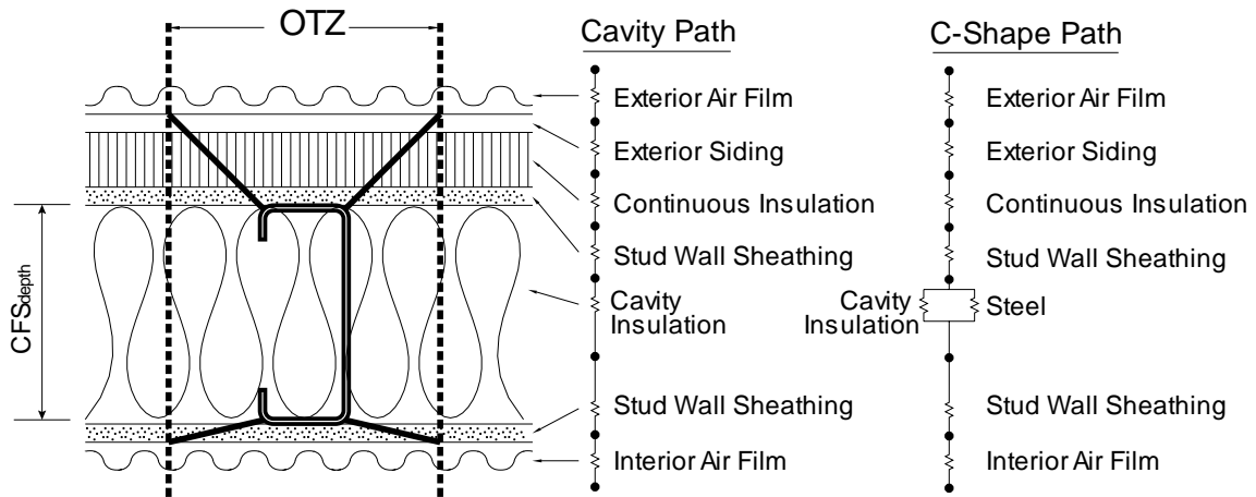
Figure B3.1.3-1 Wall Assembly and Circuit Diagram - Without Cavity Air Space
